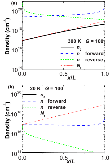
FIG. 2. (Color online) Theoretical free electron distributions for equilibrium state ( n_0 ) and forward and reverse bias ( n ) for a given N_t (dashed-dotted lines), N_A^-(x) = 0.01N_t(x) , E_C - E_V = 20 meV, N_{C0} = 10^{19} \text{ cm}^{-3} (300 K) and J = 10^3 q^2 \mu n_0^2(0) L / \epsilon . The solid, dashed, and short dashed lines correspond to n_0 , n for forward and reverse bias, respectively.
