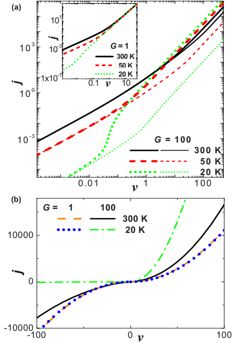
FIG. 7. (Color online) (a) Temperature dependence of J - V characteristics of the forward- and reverse-bias branches by numerical solutions with E_C - E_t = 20 meV, N_A^-(x) = 0.01 N_t(x) and G = 100 with the normalization same as Fig. 5. (b) T dependence of J - V characteristics with ( G = 100 ) and without trap-density gradient ( G = 1 ): replot of J - V characteristics \pm in (a). The curves with G = 1 for T = 300 and 20 K are completely overlapped.
